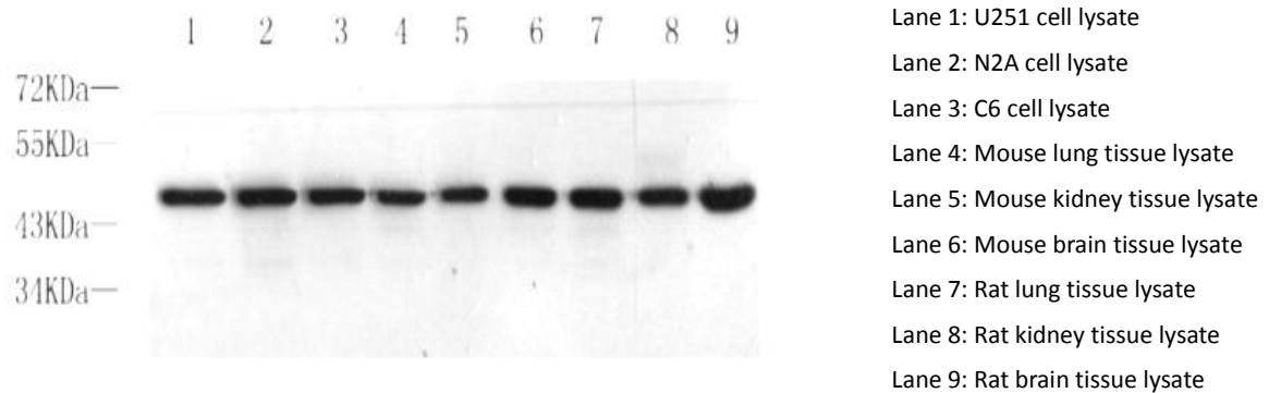
Western blot analysis of \beta -Actin at dilution of 1:2000.
